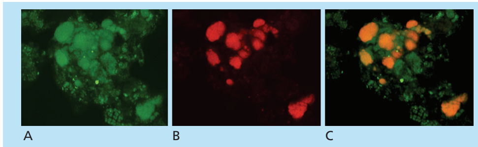
Fig. 1. This series of pictures of the same floc particle was taken using molecular probes and various microscopy techniques. A shows a floc particle from a nitrifying biomass stained green for all bacterial types. B shows the same floc particle stained red only for ammonia-oxidizing bacteria. C is an overlay of the two pictures showing the spatial distribution of nitrifiers within a well-formed floc particle.
