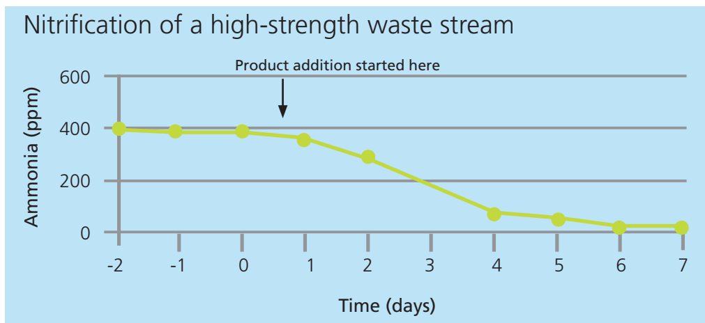
Fig. 2. Recovery of nitrification at a chemical plant.
